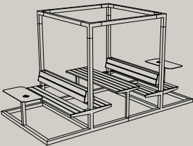
LEVP114 4335 × 2165 × 2400 one cube with terrace, benches, table and a small tables
