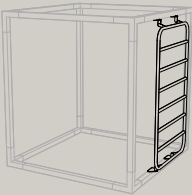
LEV900 1160 × 2240 × 224, Ø40 ladders on the wall
