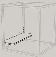
LEV320 2020 × 535 × 190 upholstered bench
