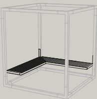
LEV315 2005 × 2000 × 75 corner wooden bench
