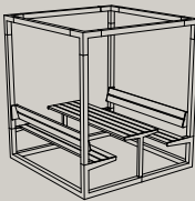
LEVP110 2165 × 2165 × 2400 one cube with benches and a table
