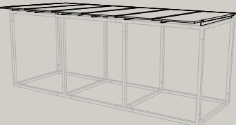
LEV413 2105 × 2976 x 134 sandwich panel roof
